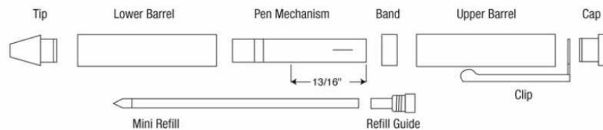
Diagram C - Assembly
